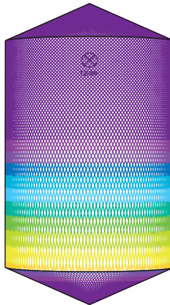
D2m H3m, Toftejorg TZ-89, 4 x ϕ4 mm Time = 11.1 min., Water consumption = 637 l
