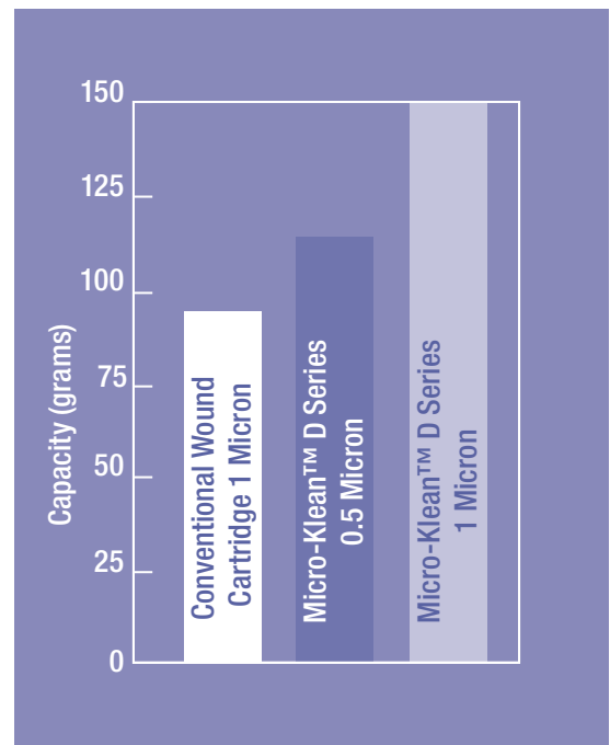
Graph 2 – Service Life
