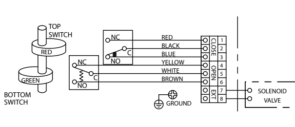
(2) SPDT SWITCHES
