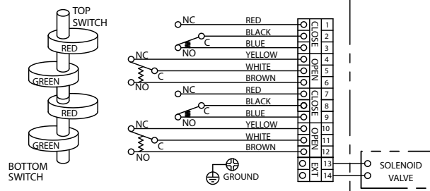
(4) SPDT SWITCHES
