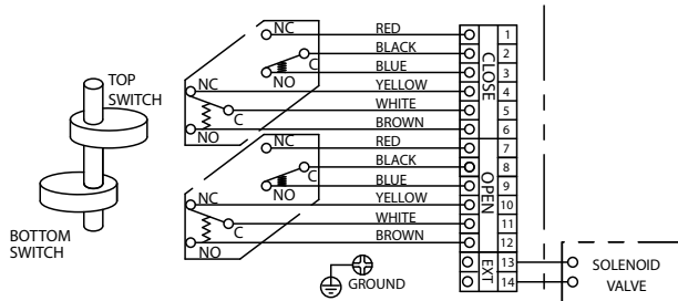
(2) DPDT SWITCHES
