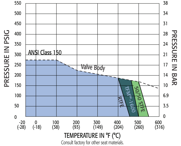
Pressure vs. Temperature Chart for Class 150 Flanged Valves 1-1/2" to 6"
