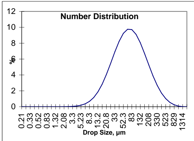
TF24FCN at 40 psi
