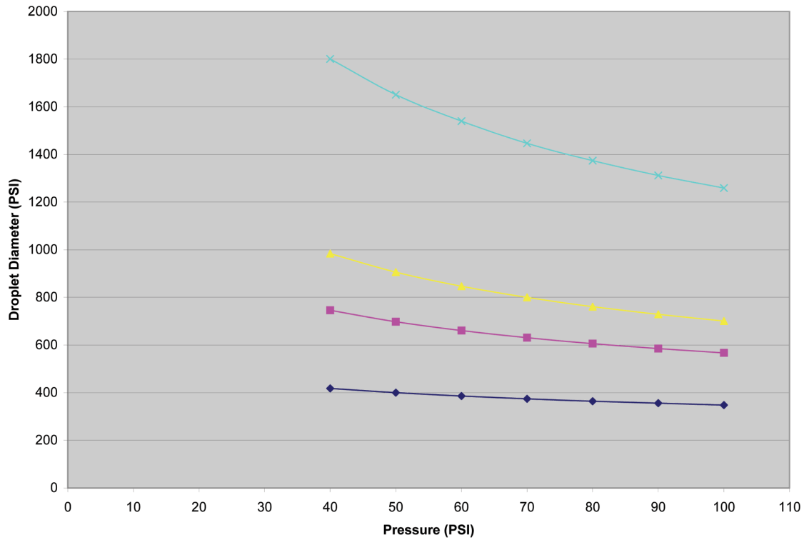
Droplet Diameters as Function of Water Delivery Pressure
