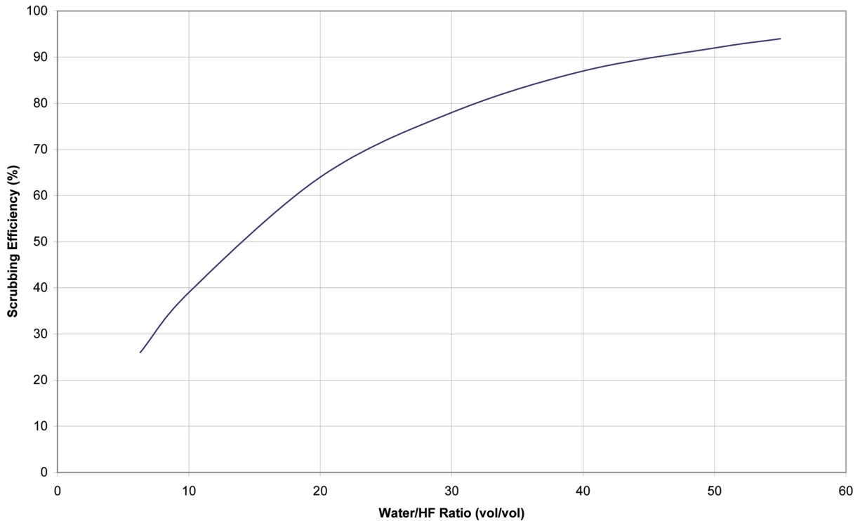
Figure 1. Field HF Water Spray Study, base case
