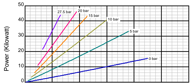
Viscosity: 1,000 cst
