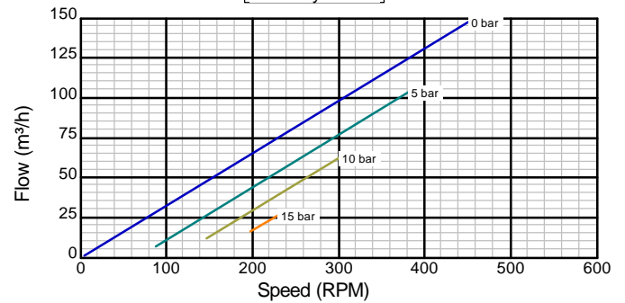
Viscosity: 21 cst
