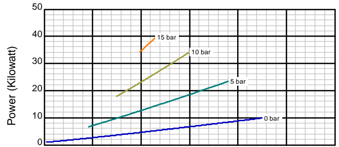
Viscosity: 21 cst
