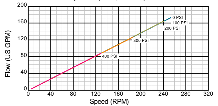
[Viscosity: 500,000 SSU]
