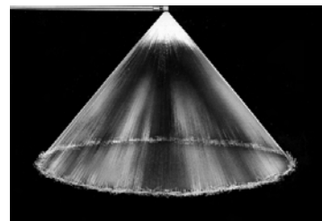
90° Hollow Cone
