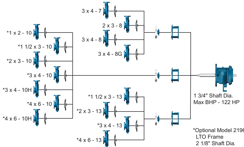
Model 2196 MTO
